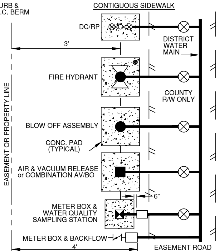
TYPE "D" INSTALLATION UNIMPROVED AREA
