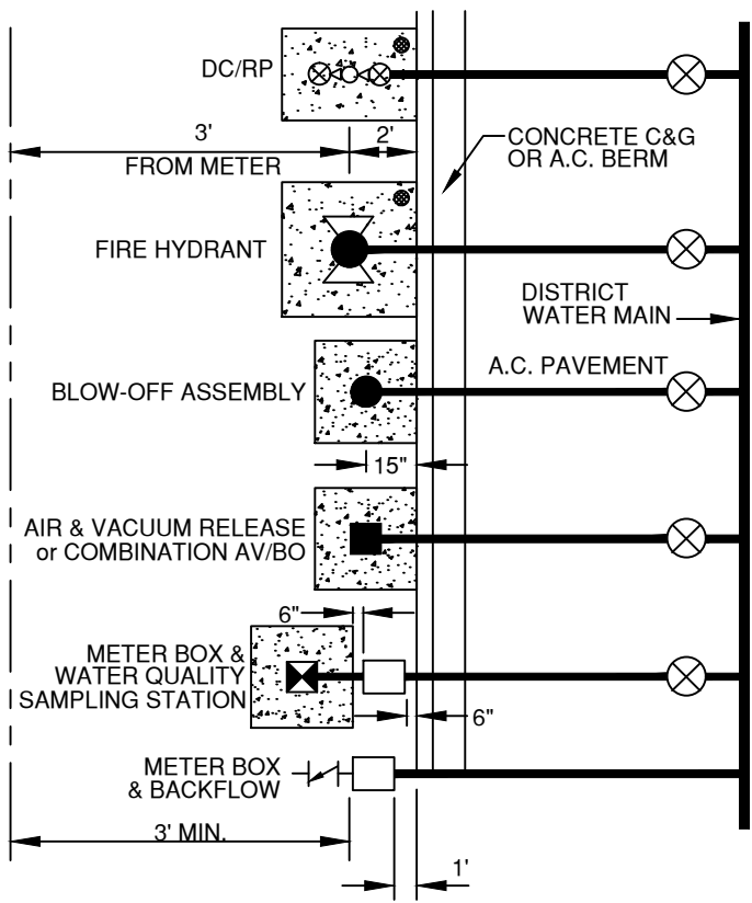
TYPE "A" INSTALLATION IMPROVED ROADWAY
